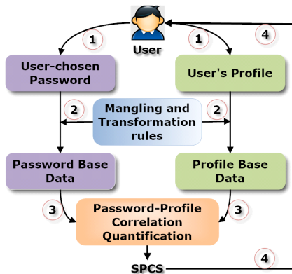
Fig. 4. Architecture of SocialShield.
