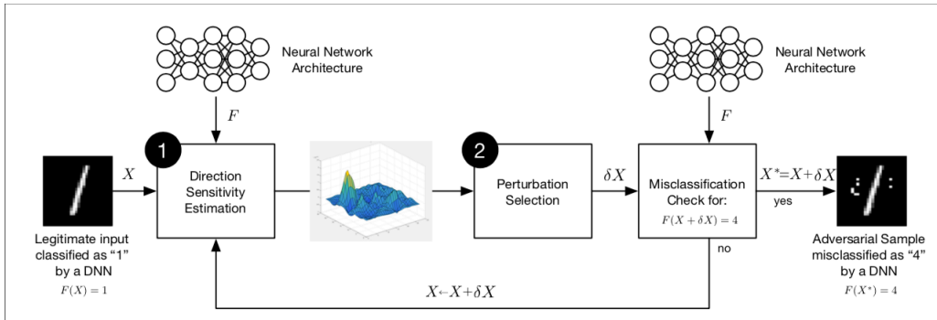
Fig.3 Adversarial example crafting framework
