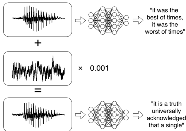
Fig.6 Illustration of targeted adversarial audios
