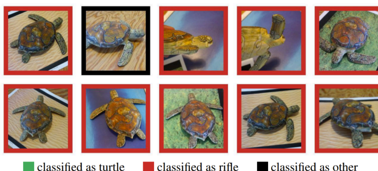
Fig.4 Different random poses of a 3D-printed turtle perturbed by EOT are classified
