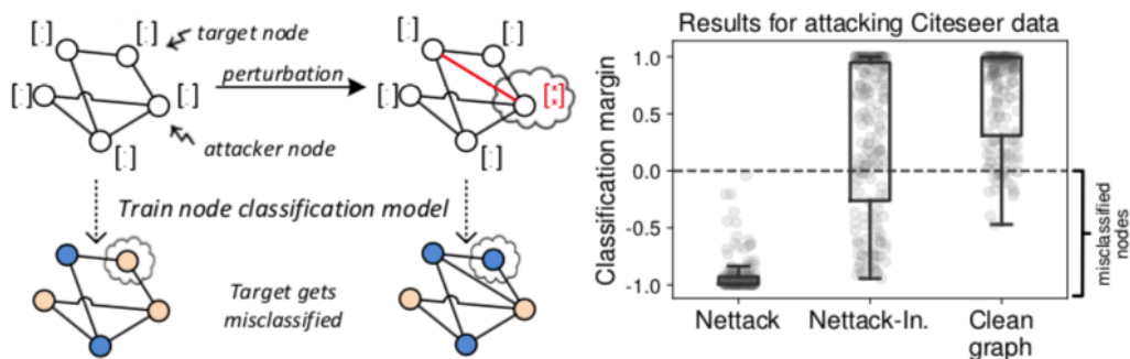
Fig.7 Small perturbations of the graph structure and node features lead to misclassification of the target model
