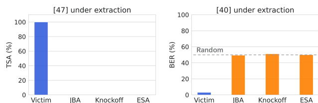
Fig. 12: Existing watermarking methods [47] and [40] failed to verify the ownership of the extracted models by several extraction attacks.
