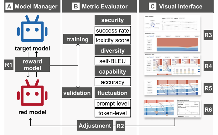
Fig. 1: System Overview: The system includes a model manager (A), a metric evaluator (B), and a visual interface (C). The models feature an automatic training paradigm (R1), and the metrics and visualizations uncover the performance and patterns in the dynamic training and validation phases (R3-R6). With the visual interface, experts can further adjust the model to achieve better model performance.
